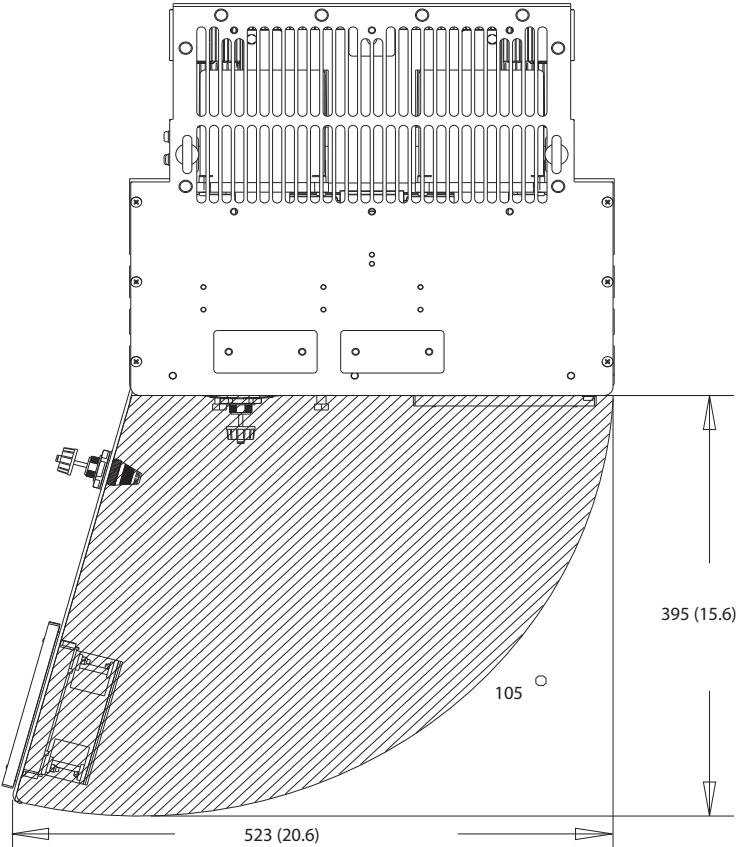
Illustration 8.29 Door Clearance for D5h
